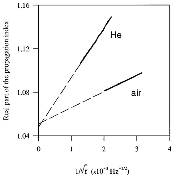
FIG. 2. Real part of the propagation index as a function of the square root of the inverse frequency.
