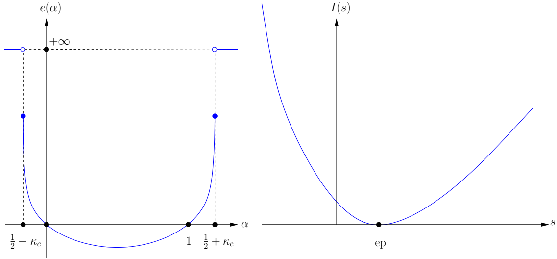
Figure 4: The cumulant generating function e(\alpha) and the rate function I(s) for the canonical entropic functional of a harmonic network satisfying Assumption (C) and ep > 0 . Notice the bias due to the symmetry I(-s) = I(s) + s .
