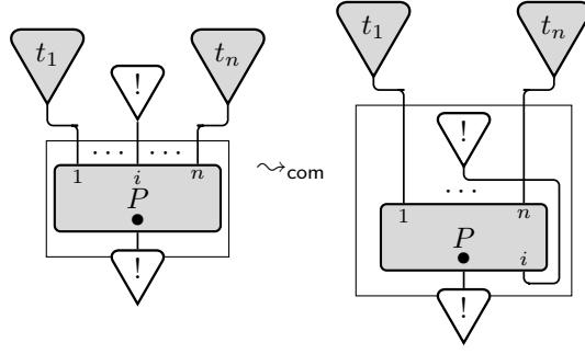
Figure 16: Promotion/coweakening commutative reduction
