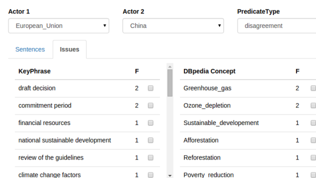
Figure 6: The AgreeDisagree View displays keyphrases and DBpedia concepts found in sentences where selected actors (here The EU and China) agree or disagree.
