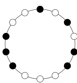
(b) Configuration \mathcal{C}' computed from \mathcal{C} by applying REDUCE 1 .
