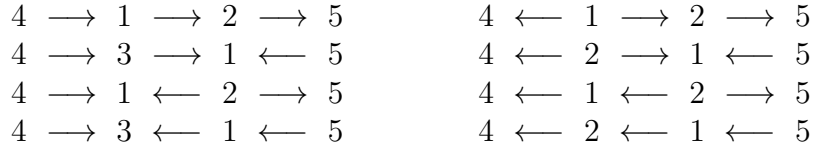
Figure 1: Coloring of oriented paths of length 3 (proof of Theorem 21)
