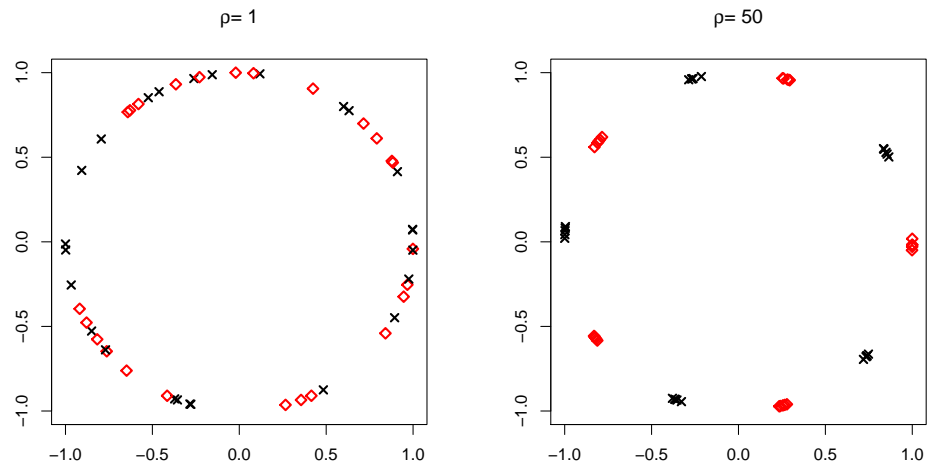
Figure 1: Two data sets are generated with two different values for the parameter \rho to highlight the influence of this parameter. Two clusters of five data are represented on each plot. Each data is composed of k = 5 angles on the circle. One cluster is represented by the black cross, the other by the red square.
