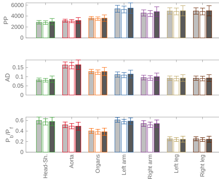
Figure 8. Pulse pressure ( PP_{[Pa]} ), area distensibility (AD) and reflection magnitude ( RM = P_b/P_f ) statistics (mean \pm std) averaged by main cardiovascular groups. Light gray bars refer to the case of cardiovascular uncertainty modeling, while white (respectively dark gray) bars refer to the augmented case including proximal (respectively proximal-distal) aortic distensibility uncertainty modeling (see section 3.3).
