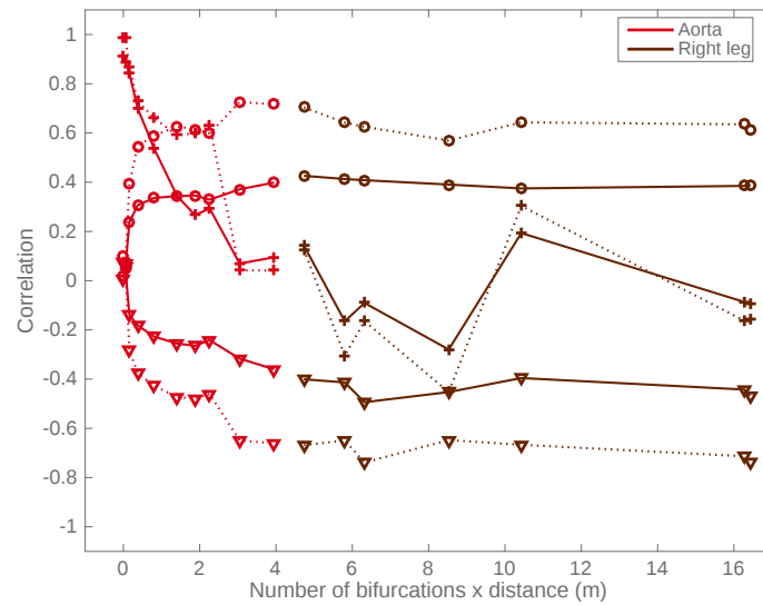
Figure 19. Correlation coefficients \rho_{RM,T} (+), \rho_{RM,\bar{Q}} ( \nabla ) and \rho_{RM,Q_{max}} (o) along part of the arterial network. Dotted lines refer to the case of cardiovascular uncertainty modeling alone, while solid lines refer to the augmented case accounting for proximal-distal aortic distensibility uncertainty modeling.
