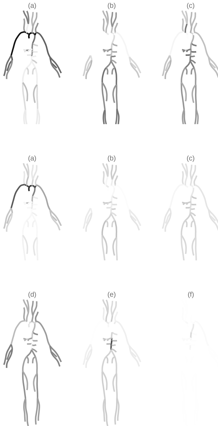
Figure 18. Detailed RM first-order Sobol' indices: S_T (a), S_{\overline{Q}} (b), S_{Q_{max}} (c), S_{c_{01}} (d), S_{c_{02}} (e) and S_{c_{03}} (f) for Case 2 . Low (respectively high) values are represented in white (respectively black) color.
