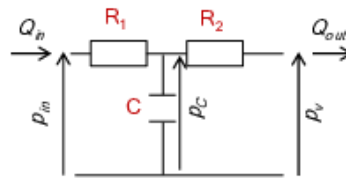
Figure 2. Electric circuit analogy with lumped 0D RCR Windkessel model.
