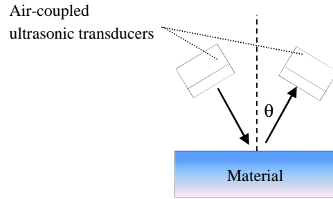
Fig. 6. Principle of the measurement of kinematic porosity and tortuosity from reflected ultrasonic waves. At least two measurements with two different angles are necessary.
