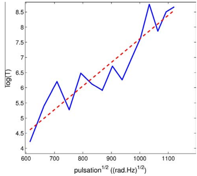
Fig. 5. Logarithm of the transmission coefficient as a function of the square root of the angular frequency for sample 2. The intercept of the straight line with the vertical axis (at 0 Hz) leads to the kinematic porosity.
