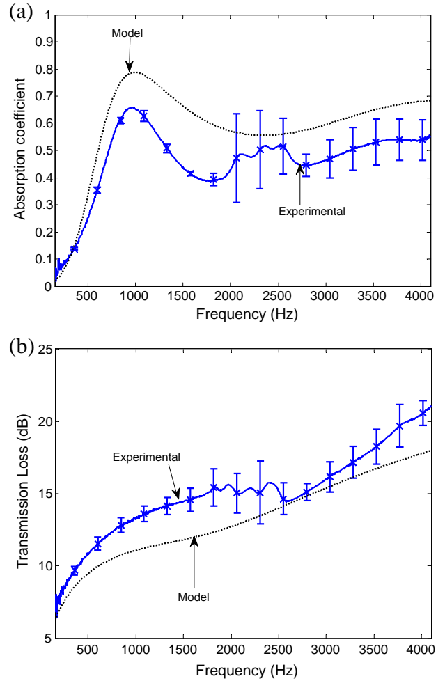
Fig. 10. Comparison between the experimental results and the theoretical predictions for (a) the absorption coefficient and (b) the transmission loss.
