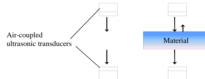
Fig. 4. Principle of the measurement of kinematic porosity from the logarithm of the transmission coefficient \ln(T) [15].
