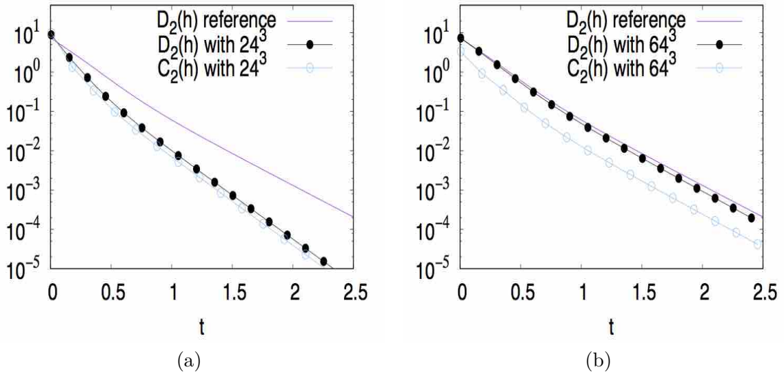
FIGURE 4. Fokker-Planck equation with an external magnetic field. Time evolution of the physical dissipation and the numerical dissipation ( D_2(h), C_2(h) ) corresponding to the entropy H_2(h) with (a) N = 24^3 mesh points (b) N = 64^3 mesh points.
