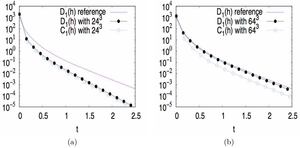
FIGURE 3. Fokker-Planck equation with an external magnetic field. Time evolution of the physical dissipation and the numerical dissipation ( D_1(h), C_1(h) ) corresponding to the entropy H_1(h) with (a) N = 24^3 mesh points (b) N = 64^3 mesh points.
