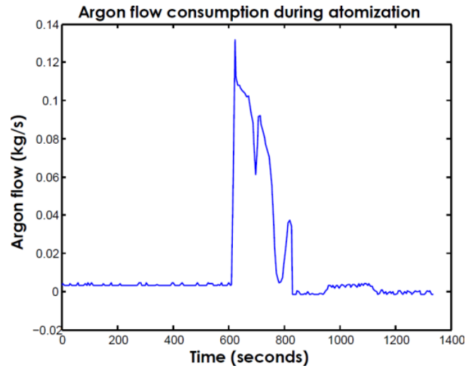
Figure 21. Argon flow consumption.
