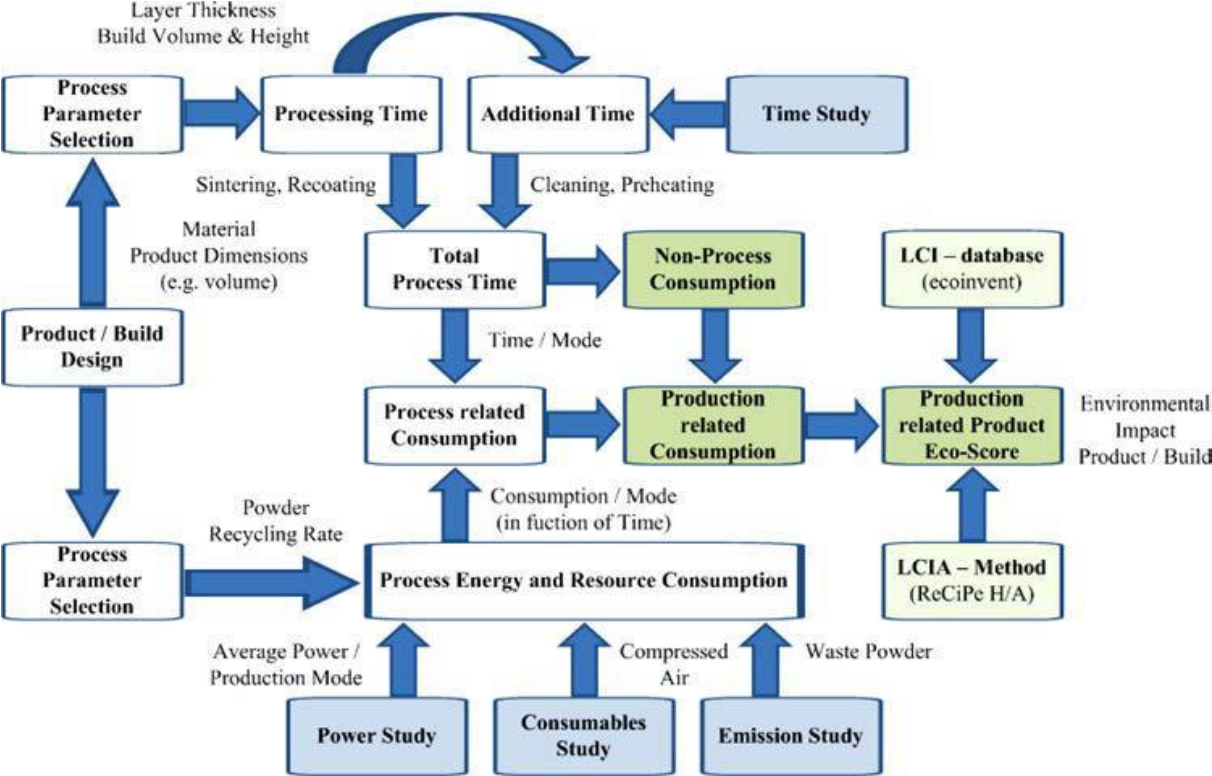
Figure 13. Overview of the parametric impact estimation model for SLS process [31].
