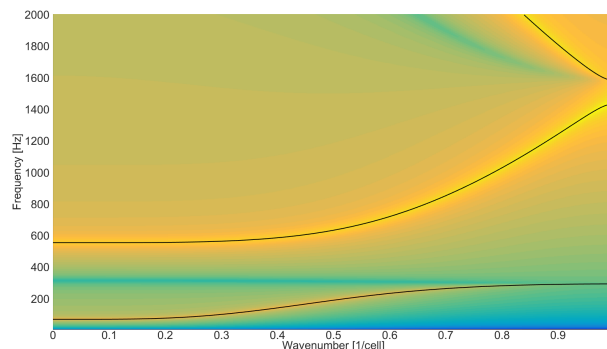
Figure 4: Amplitude of the forced response of a periodic track in the wavenumber/frequency domain.
