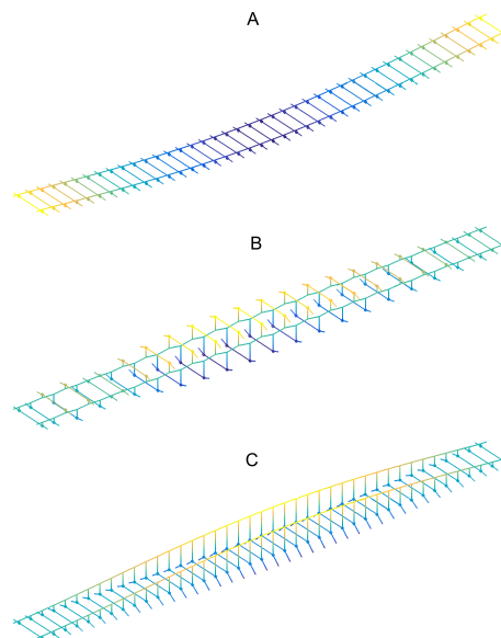
Figure 5: Finite length modes associated with points A,B,C
