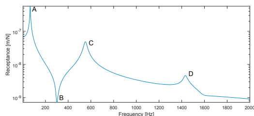
Figure 3: Receptance associated with an impact on the rail.
