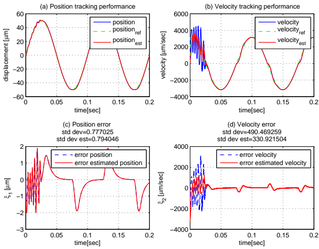
Fig. 5. Trajectory tracking performance @ 10hz
