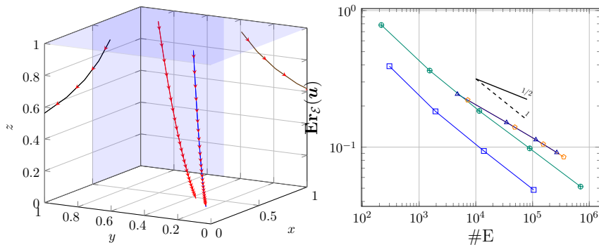
Figure 5: Left panel: inflow boundary \partial\Omega^- in blue and some streamlines of the vector field \boldsymbol{\beta} . Right panel: Discrete errors on H ( \square ), PrT ( \triangle ), PrG ( \diamond ), and CB ( \oplus ) mesh sequences.
