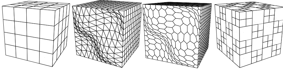
Figure 4: Examples of meshes from the four sequences. From left to right: hexahedral mesh (H), prismatic mesh with triangular basis (PrT), prismatic mesh with hexagonal basis (PrG), and Checkerboard mesh with non-matching interfaces (CB).
