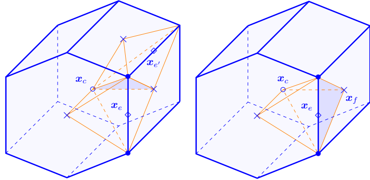
Figure 2: In blue. Left: intra-cell sub-face \mathfrak{f} = \partial\mathfrak{p}_{e,c} \cap \partial\mathfrak{p}_{e',c} \in \mathfrak{F}_c . Right: inter-cell sub-face \mathfrak{f} = \partial\mathfrak{p}_{e,c} \cap \partial\mathfrak{p}_{e',c'} \in \mathfrak{F}_f .
