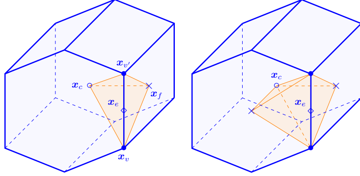
Figure 1: Left panel: tetrahedron [\mathbf{x}_v, \mathbf{x}_{v'}, \mathbf{x}_f, \mathbf{x}_c] . Right panel: local diamond \mathfrak{p}_{e,c} .
