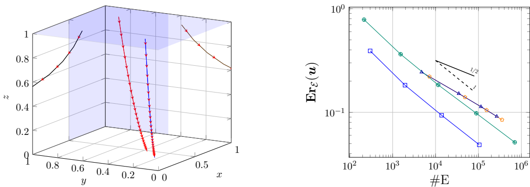
Figure 5: Left panel: inflow boundary \partial\Omega^- in blue and some streamlines of the vector field \boldsymbol{\beta} . Right panel: Discrete errors on \mathbf{H} ( \square ), \mathbf{PrT} ( \triangle ), \mathbf{PrG} ( \circ ), and \mathbf{CB} ( \oplus ) mesh sequences.
