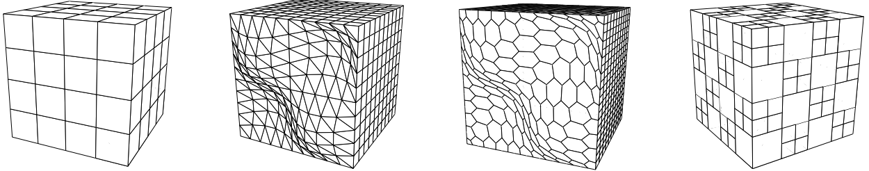
Figure 4: Examples of meshes from the four sequences. From left to right: hexahedral mesh ( \mathbf{H} ), prismatic mesh with triangular basis ( \mathbf{PrT} ), prismatic mesh with hexagonal basis ( \mathbf{PrG} ), and Checkerboard mesh with non-matching interfaces ( \mathbf{CB} ).
