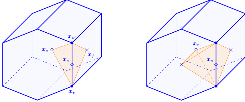
Figure 1: Left panel: tetrahedron [\mathbf{x}_v, \mathbf{x}_{v'}, \mathbf{x}_f, \mathbf{x}_c] . Right panel: local diamond \mathfrak{p}_{e,c} .
