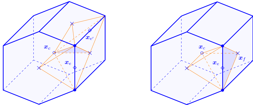
Figure 2: In blue. Left: intra-cell sub-face \mathfrak{f} = \partial\mathfrak{p}_{e,c} \cap \partial\mathfrak{p}_{e',c} \in \mathfrak{F}_c . Right: inter-cell sub-face \mathfrak{f} = \partial\mathfrak{p}_{e,c} \cap \partial\mathfrak{p}_{e',c'} \in \mathfrak{F}_f .
