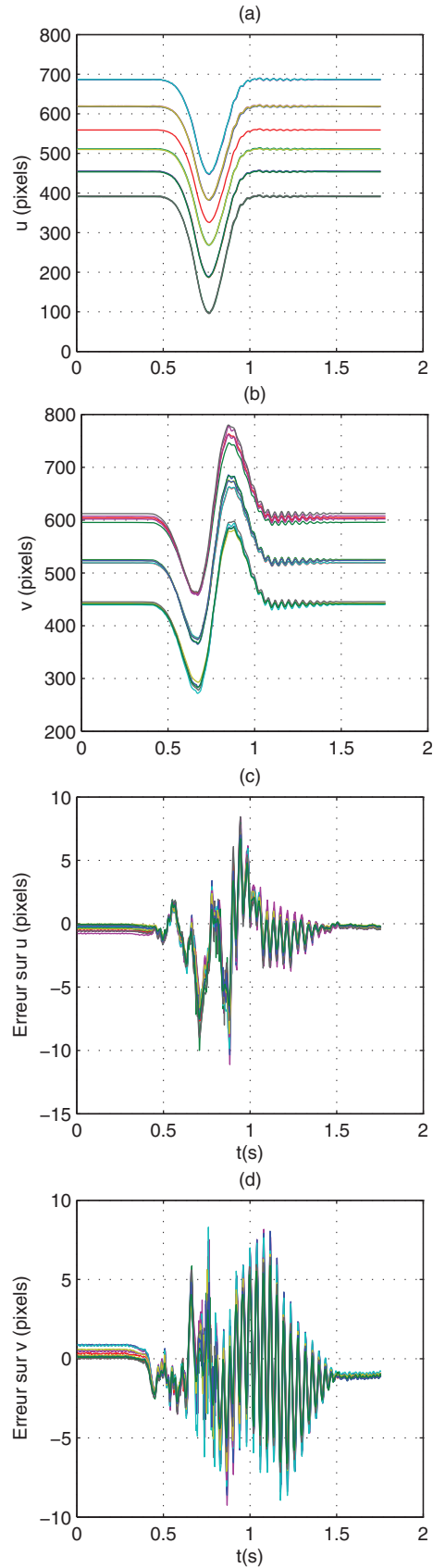
Fig. 17. Features positions in the image along (a) the $u$-axis and (b) the $v$-axis, and the positions errors along (c) the $u$-axis and (d) the $v$-axis for a control angular frequency of 50 \text{ rad s}^{-1} .
