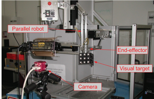
Fig. 6. Experimental setup for position-based and image-based visual servos on the Orthoglide.
