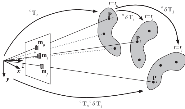
Fig. 1. Projection model of a set of points in the case of sequential acquisition. At the time instant t_0 , the relative pose between the object and the robot is {}^c\mathbf{T}_o . The relative pose at t_i and t_j are, respectively, {}^c\mathbf{T}_o \delta\mathbf{T}_i and {}^c\mathbf{T}_o \delta\mathbf{T}_j which means that the projected points do not correspond to the same pose of the object.
