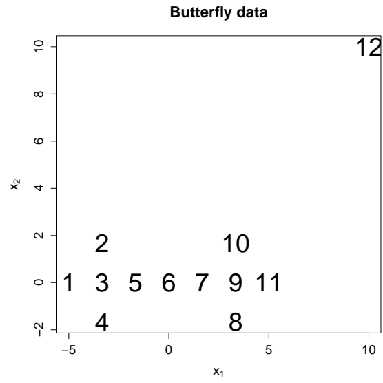
Figure 1: Butterfly dataset.
