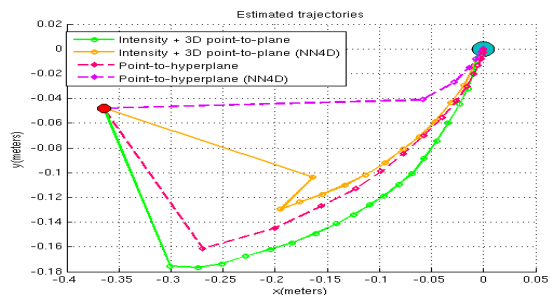
Fig. 4. Example of 4 estimated camera trajectories between a pair of images with a random pose in a simulated environment. The green and red dot indicate the initial and the final pose. The Point-to-hyperplane methods improve the Point-to-plane + direct methods, obtaining more direct trajectories when NN4D are estimated. 1000 synthesized images with a random pose were equally tested, obtaining a similar performance.
