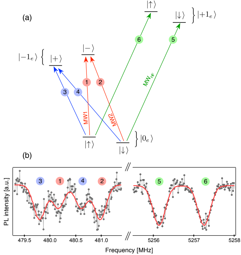
FIG. 5: (a)-Energy level structure of the spin system showing the nuclear spin eigenstates in the m_s = 0 ( |0_e\rangle ) and m_s = \pm 1 ( |±1_e\rangle ) electron spin manifolds. We consider \mathcal{A}_{zz} \sim \gamma_n B and \mathcal{A}_{zz} > 0 . The colored arrows indicate electron spin transitions labelled from ① to ⑥. (b)-ESR spectrum recorded for the coupled spin system with a magnetic field B = 850 G applied along the NV defect axis. The low frequency part of the spectrum is reproduced from Fig. 1 of the main text.
