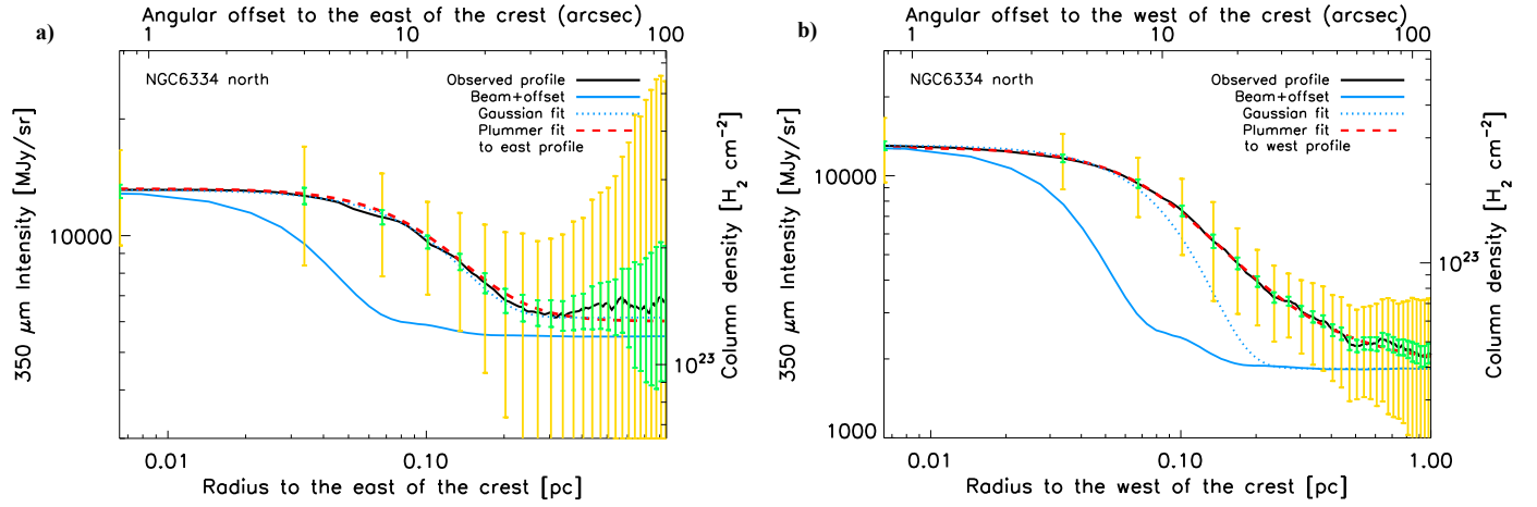
Fig. A.1. a) Median radial intensity profile of the northern part of the NGC 6334 filament (black solid curve) measured in the combined ArTéMiS + SPIRE 350\ \mu\text{m} image (Fig. 1b) perpendicular to, and on the eastern side of, the filament crest shown as a white curve in Fig. 2a. The yellow and green error bars are as in Fig. 3a. The blue solid curve shows the effective beam profile of the ArTéMiS 350\ \mu\text{m} data as measured on Mars, overlaid on a constant level corresponding to the typical background intensity level observed at large radii. The blue dotted curve shows the best-fit Gaussian (+ constant offset) model to the inner part of the observed profile. The red dashed curve shows the best-fit Plummer model convolved with the beam (cf. Sect. 3 and Eq. (2)). b) Same as in a) but for the median radial intensity profile of the northern part of the filament measured on the western side of the filament crest shown as a white curve in Fig. 2a.
