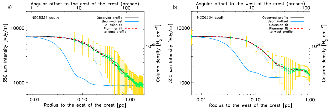
Fig. A.2. a) Median radial intensity profile of the southern part of the NGC 6334 filament (black solid curve) measured in the combined ArTéMiS + SPIRE 350\ \mu\text{m} image (Fig. 1b) perpendicular to, and on the eastern side of, the filament crest shown as a magenta curve in Fig. 2a. The yellow and green error bars are as in Fig. 3a. The blue solid curve shows the effective beam profile of the ArTéMiS 350\ \mu\text{m} data as measured on Mars, overlaid on a constant level corresponding to the typical background intensity level observed at large radii. The blue dotted curve shows the best-fit Gaussian (+ constant offset) model to the inner part of the observed profile. The red dashed curve shows the best-fit Plummer model convolved with the beam (cf. Sect. 3 and Eq. (2)). b) Same as in a) but for the median radial intensity profile of the southern part of the filament measured on the western side of the filament crest shown as a magenta curve in Fig. 2a.
