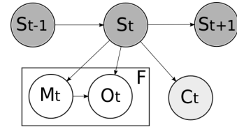
Fig. 3: Graphical Model of the framework for handling missing data. S_t is the hidden state, M_t represents whether an observation has been made or not, O_t is the corresponding observation, and C_t is the associated class. F is the number of features considered. Light grey : variables that are accessible solely during the learning phase. Dark grey : variables that are never accessible.
