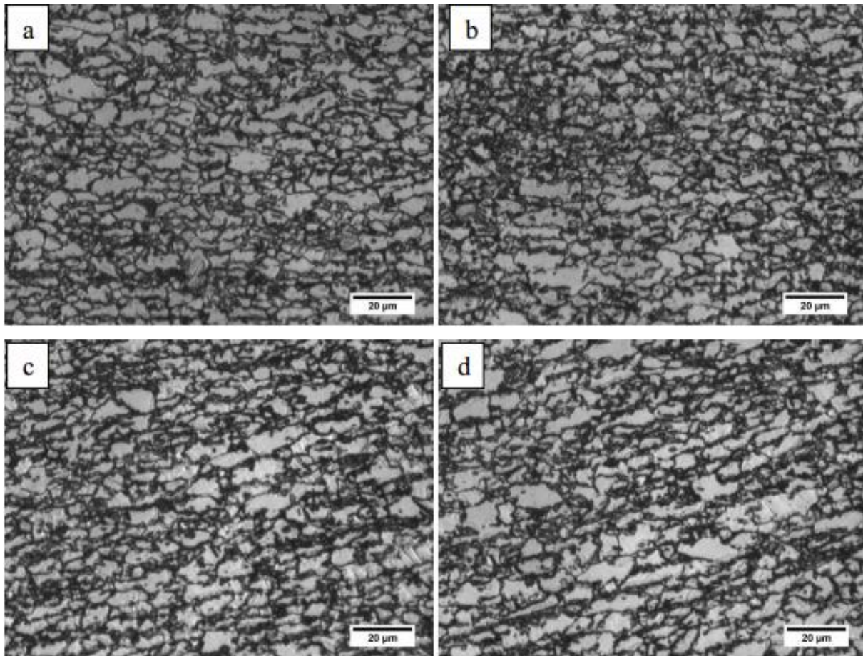
Fig. 7. Optical microscopy images dual-phase steel as received and subjected to mechanical bending, where (a) and (b): material as received; (c) and (d): 120°, increase of 500X, reagent Nital 2%.
