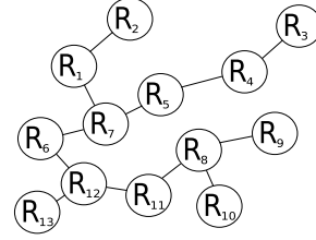
Figure 4: Minimum Spanning Tree: the distance between two regions corresponds to the number of edges of the shortest path connecting them. E.g., dist(R_5, R_7) = 1 , dist(R_{56}, R_4) = dist(R_5, R_4) + dist(R_6, R_4) = 4 and dist(R_{56}, R_{49}) = 5 .
