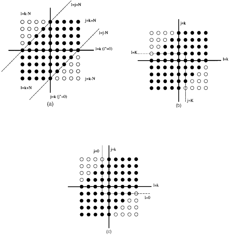
Figure 1. Structure of \Lambda_{j'',k''} index pad for 3-tuples in the (j, l) plane: (a) the index pad corresponds to N=4 in the region where no wraparound arises; (b) corresponding to N=4 for k=k'+2 ; (c) corresponding to N=4 for k=N-3 , \sigma=2
