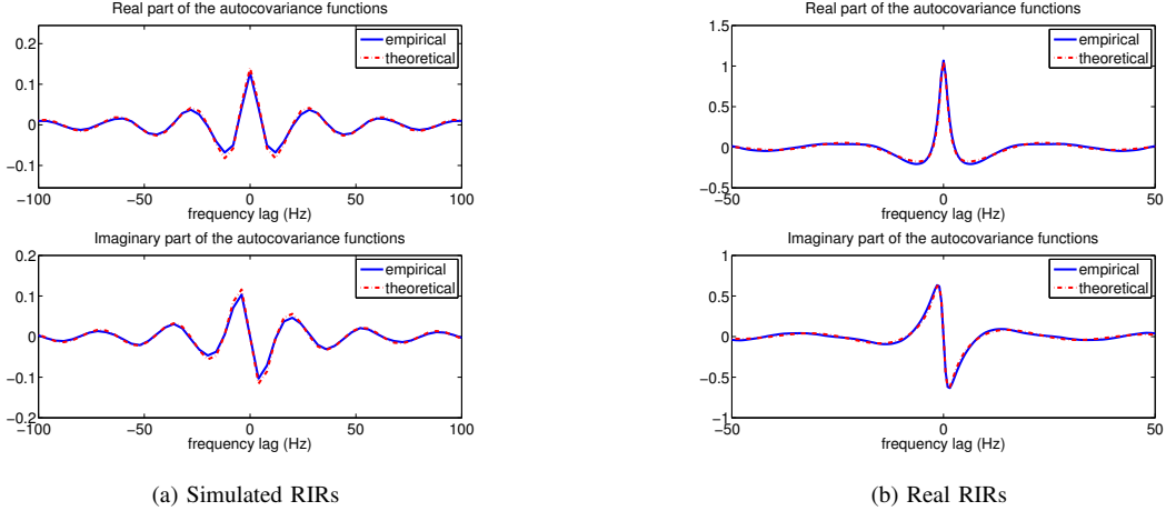
Fig. 2: Theoretical and empirical ACVFs.
