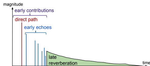
Fig. 1: Schematic illustration of a room impulse response.
