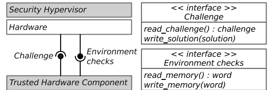
Fig. 2: Security architecture hardware interfaces
