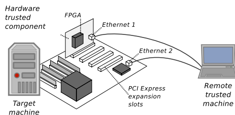
Fig. 4: Security architecture platform
