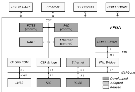
Fig. 6: System on chip
