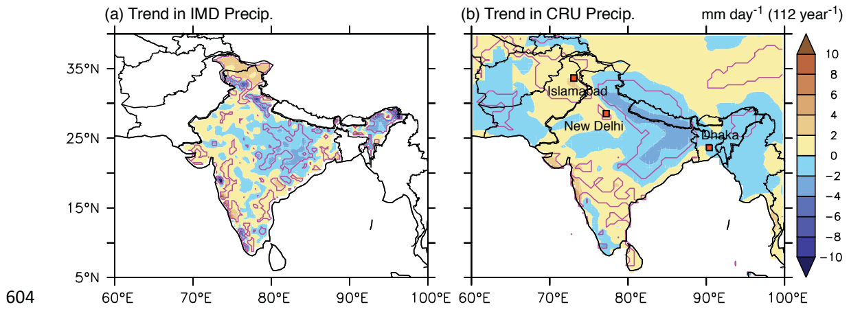
604 605 Figure 1. Observed trend in precipitation (mm day -1 112 year -1 ) in (a) IMD and (b) CRU datasets, during 606 June-September, for the years 1901-2012. Contours denote regions significant at the 95% confidence 607 level.
