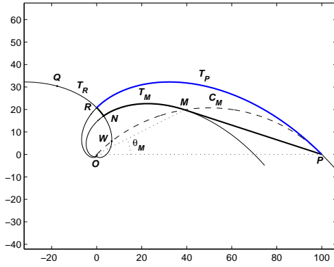
Fig. 2. Example of new path of type T2_Q * T1 - SL .
