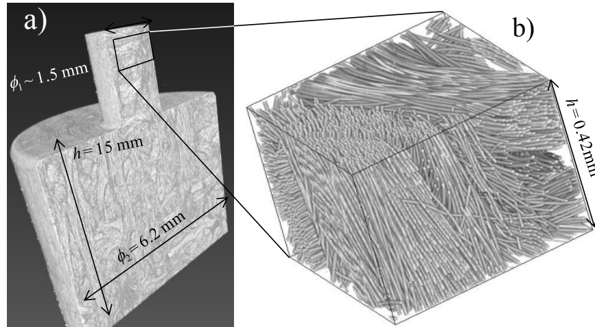
Figure 1. 3D renderings of \mu\text{-CT} scans of a partly infiltrated C/C sample shaped for CT acquisition at 2 distinct resolutions. a) Low-resolution scan. b) High-resolution image, after segmentation from an edge-detection mode scan.
