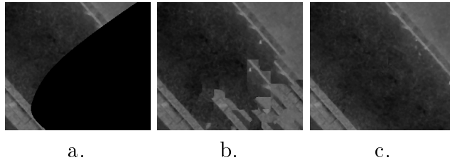
Figure 7: Comparison of (16) and our proposed modification on the junction between the road and a pavement. (a) is the original unfilled image where the dark region is being reconstructed using exemplar-based inpainting, (b) the result from (16), (c) our proposed optimization. The result is clearly better in (c) as the reconstruction conserves the structures of the image without creating new artifacts such as the one appearing on the left of (b).
