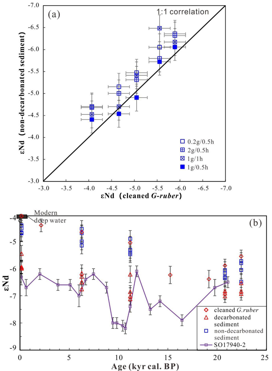
Figure 6. (a) Crossplot of \epsilon_{Nd} values of non-decarbonated sediment leachates and \epsilon_{Nd} values obtained from cleaned planktonic foraminifera G. ruber . (b) \epsilon_{Nd} values obtained from acid-reductive HH leachates of bulk non-decarbonated and decarbonated sediments of core MD05-2904. \epsilon_{Nd} values have been obtained by using HH leaching of 0.2, 1, and 2 g samples of sediments leached for 0.5, 1, 2, and 3 h. \epsilon_{Nd} obtained on seawater samples close to the studied site [Wu et al. , in press] as well on cleaned planktonic foraminifera G. ruber of core MD05-2904 are also reported. \epsilon_{Nd} from acid-reductive HH leachates of bulk decarbonated sediments of the core SO17940-2 [Huang et al. , 2013] are also reported for comparison.
