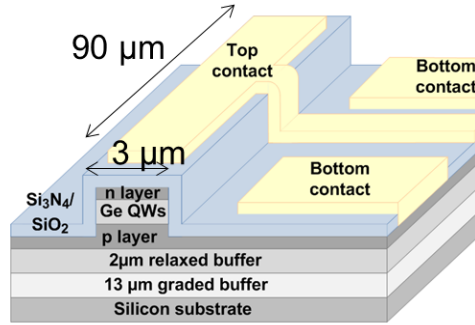
Fig. 1. Schematic view of a Ge/SiGe QW structure in a waveguide configuration that can be used as a modulator or as photodetector.
