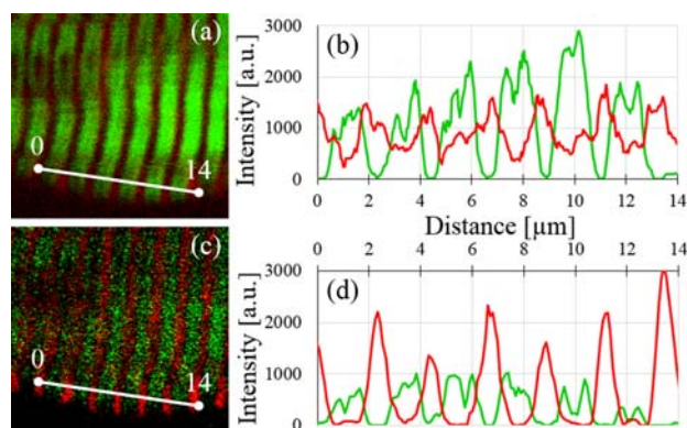
Figure 4 TPF (red) and SHG (green) intensity profiles plotted along the line drawn in (a) and (c) respectively under (b) nanosecond SC and (d) femtosecond Ti:Sa excitation.
