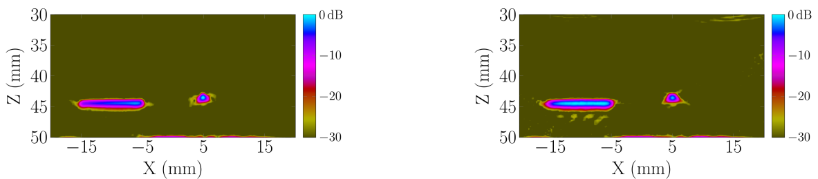
Fig. 5. Experimental images obtained with the (a) STA (64 transmissions). (b) PWI (9 transmissions).
