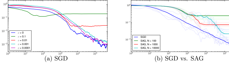
Figure 2: (a) Plot of \|\mathbf{v}_k - \mathbf{v}_0^*\|_2 / \|\mathbf{v}_0^*\|_2 as a function of k , for SGD and different values of \epsilon ( \epsilon = 0 being un-regularized). (b) Plot of \|\mathbf{v}_k - \mathbf{v}_\epsilon^*\|_2 / \|\mathbf{v}_\epsilon^*\|_2 averaged over 40 runs as a function of k , for SGD and SAG with different number N of samples, for regularized OT using \epsilon = 10^{-2} .
