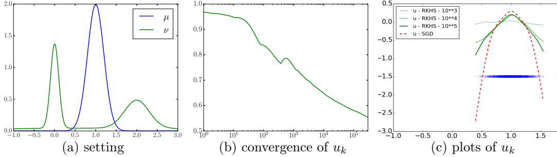
Figure 3: (a) Plot of \frac{d\mu}{dx} (blue) and \frac{d\nu}{dx} (green). (b) Plot of \|\mathbf{u}_k - \hat{\mathbf{u}}^*\|_2 / \|\hat{\mathbf{u}}^*\|_2 as a function of k with SGD in the RKHS, for regularized OT using \varepsilon = 10^{-1} . (c) Plot of the iterates u_k for k = 10^3, 10^4, 10^5 and the proxy for the true potential \hat{\mathbf{u}}^* , evaluated on a grid where \mu has non negligible mass.
