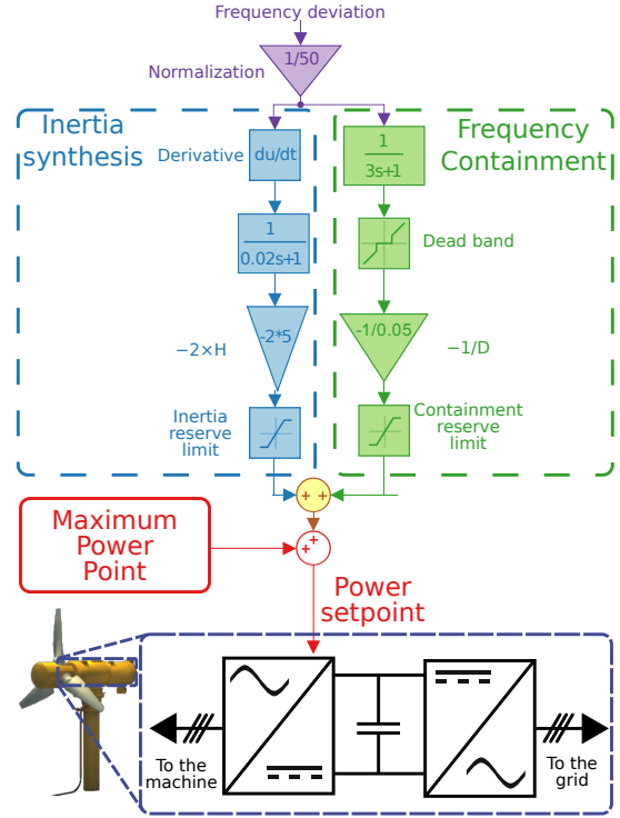
Fig. 5. Structure of the two controls (inertia and containment): example of an individual tidal turbine with a back-to-back AC/DC/AC converter
