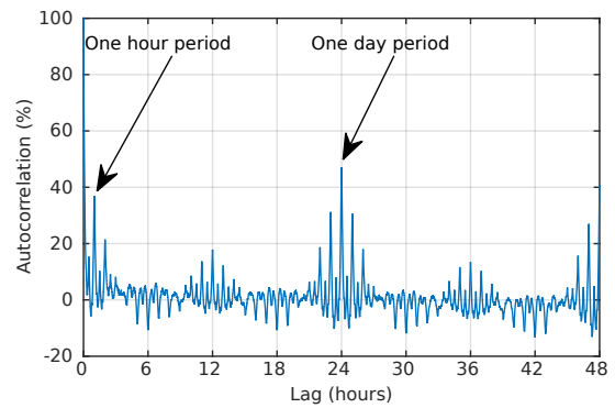
Fig. 9. Autocorrelation of the frequency deviation signal
