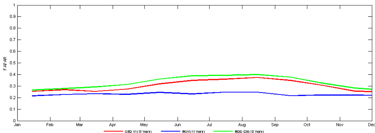
Figure 8. Average global seasonality computed for the three products: GEOV1 (red), MGVIo (blue) and MODC5 (green). Products are displayed at their original temporal resolution (Table 2). The 49 × 49 pixel values are averaged over all the BELMANIP2 sites, and then averaged over years for the period defined in the validation exercise.
