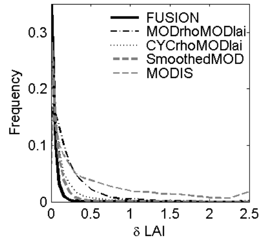
Fig. 6. Histogram of the \delta absolute value for the original and the developed MODIS LAI products.
