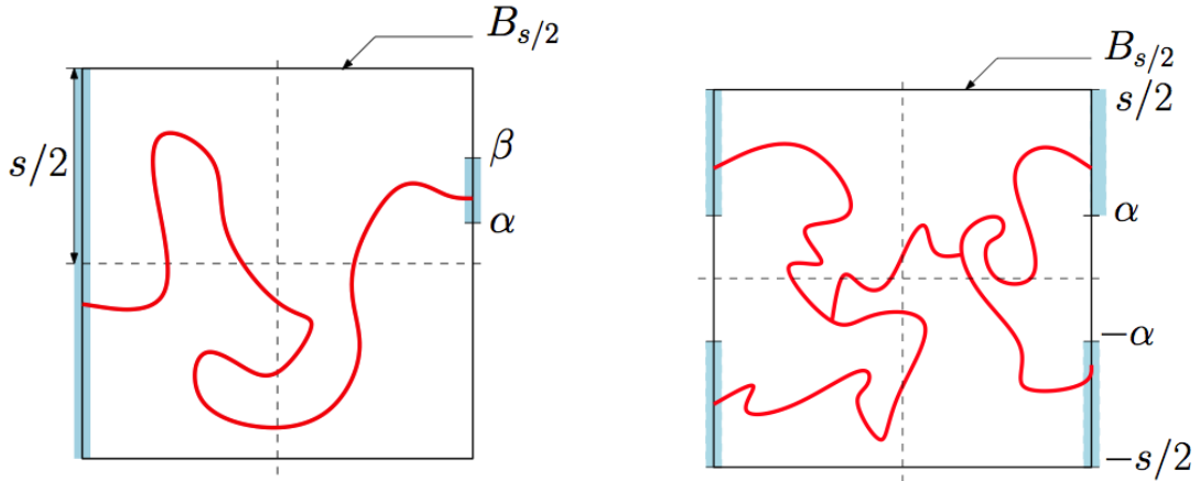
Fig. 2.2. The events \mathcal{H}_s(\alpha, \beta) and \mathcal{X}_s(\alpha) (from [40])
