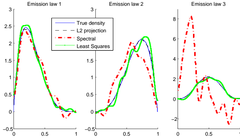
Figure 6: Estimators of the emission densities for n = 19,998 and Beta parameters (2; 5) , (4; 2) and (4; 4) . We took K = \hat{K}_{1,s} = 3 and M = \hat{M} = 13 . The bad behaviour of the spectral algorithm when the emission densities are poorly separated is clearly visible on the third emission distribution.
