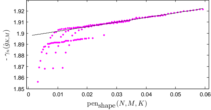
Figure 4: Empirical constraint and calibrated penalty for n = 49,998 . Here, the parameters of the Beta distribution are (2; 5) , (4; 2) and (4; 4) .
