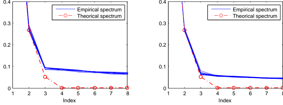
(a) n = 19,998 , Beta parameters (2; 5) , (4; 2) and (4; 4) . (b) n = 49,998 , Beta parameters (2; 5) , (4; 2) and (4; 4) .
