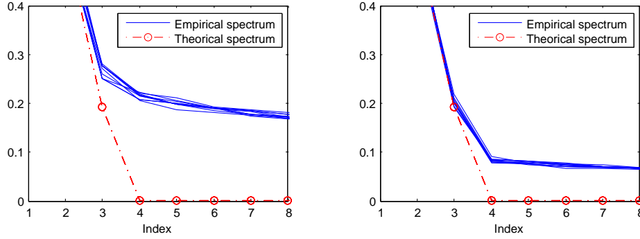
(c) n = 3,000 , Beta parameters (1.5; 5) , (7; 2) and (6; 6) . (d) n = 19,998 , Beta parameters (1.5; 5) , (7; 2) and (6; 6) .
