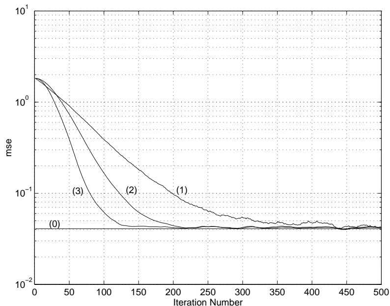
Figure 2 Learning curves of the mean square error E(\|\mathbf{P}(k) - \mathbf{P}_* \|_{\text{Fro}}^2) averaging 100 independent runs for the Oja's algorithm (1) and the smoothed Oja's algorithm with \alpha = 1 (2) and \alpha = 0.3 (3) compared with \mu \text{Tr}(\mathbf{C}_P) (0) in the same configuration (\mathbf{C}_x, \mathbf{W}(0)) that Figure 1.
