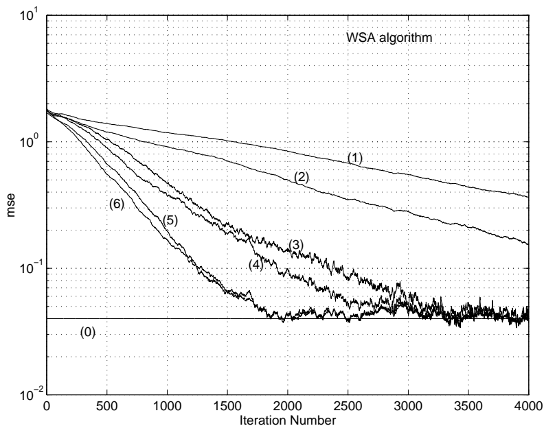
Figure 1 Learning curves of the mean square error \mathbb{E}(\|\mathbf{W}(k) - \mathbf{W}_*\|_{\text{Fro}}^2) averaging 100 independent runs for the WSA algorithm, for different values of parameter \beta_2/\beta_1 = 0.96 (1), 0.9 (2), 0.1 (3), 0.2 (4), 0.4 (5) and 0.6 (6) compared with \mu \text{Tr}(\mathbf{C}_\theta) (0) in the case n = 4 , r = 2 , \mathbf{C}_x = \text{Diag}(1.75, 1.5, 0.5, 0.25) , where the entries of \mathbf{W}(0) are chosen randomly uniformly in [0,1] .
