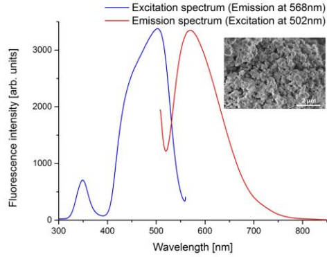
Figure 2. Emission ( \lambda_{ex} \sim 502 nm) and excitation ( \lambda_{em} \sim 568 nm) spectra of Y_3Al_5O_{12}:Ce^{3+} (3.3 % wt.) nanophosphors embedded in PDMS. The inset shows an SEM image of the nanophosphors.
