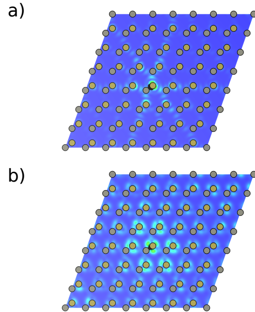
Figure 8 Slice of the excitonic wavefunction in ZnTe for a) the strongest exciton that contributes to the E_1 peak and b) the strongest exciton that contributes to the E_2 peak. View along one of the lattice vectors of 7 \times 7 \times 7 unit cells of cubic ZnTe (Zn atoms are in grey, Te atoms in olive green). The hole position is represented by a dummy atom (black) and coincides with the position of the Te in one of the unit cells. The 100 lattice plane passing through the hole position slices the excited electron wavefunction (dark blue correspond to no excited electronic density). Plots have been rendered using VESTA. 58
