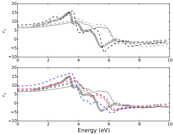
Figure 6 Real part of the macroscopic dielectric function \epsilon_1 of bulk ZnTe. Top panel: experimental spectrum 22 (circles) compared with the independent particle (grey dashed-dotted line) and random phase approximation (grey continuous line) and Bethe-Salpeter equation (black dashed line). Bottom panel: experimental spectrum (circles) compared with the approximations for the polarisation functional described in Sec. 2, \mathcal{E}^{xc} \approx \alpha^{\text{EMP}} \mathbf{P} (red dashed line), \mathcal{E}^{xc} \approx \alpha^{\text{BER}} \mathbf{P} (magenta dashed line), \mathcal{E}^{xc} \approx \alpha^{\text{ED}} \mathbf{P} (green dashed line) and \mathcal{E}^{xc} \approx \alpha^{\text{GM}} \mathbf{P} (blue dashed line). For reference the random phase approximation is also shown (grey continuous line).
