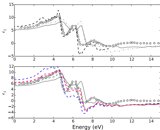
Figure 5 Real part of the macroscopic dielectric function \epsilon_1 of bulk ZnSe. Top panel: experimental spectrum 20 (circles) compared with the independent particle (grey dashed-dotted line) and random phase approximation (grey continuous line) and Bethe-Salpeter equation (black dashed line). Bottom panel: experimental spectrum (circles) compared with the approximations for the polarisation functional described in Sec. 2, \alpha^{\text{EMP}}\mathbf{P} (red dashed line), \alpha^{\text{BER}}\mathbf{P} (magenta dashed line), \alpha^{\text{ED}}\mathbf{P} (green dashed line) and \alpha^{\text{JGM}}\mathbf{P} (blue dashed line). For reference the random phase approximation is also shown (grey continuous line).
