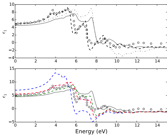
Figure 2 Real part of the macroscopic dielectric function \epsilon_1 of bulk ZnS. Top panel: experimental spectrum 20 (circles) compared with the independent particle (grey dashed-dotted line), random phase approximation (grey continuous line) and Bethe-Salpeter equation (black dashed line). Bottom panel: experimental spectrum (circles) compared with the approximations for the polarisation functional described in Sec. 2, \alpha^{\text{EMP}}\mathbf{P} (red dashed line), \alpha^{\text{BER}}\mathbf{P} (magenta dashed line), \alpha^{\text{ED}}\mathbf{P} (green dashed line) and \alpha^{\text{JGM}}\mathbf{P} (blue dashed line). For reference the random phase approximation is also shown (grey continuous line).
