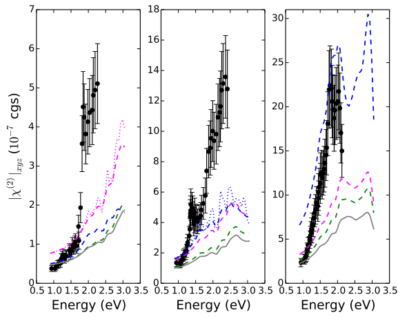
Figure 10 SHG of bulk cubic ZnS (left), ZnSe (middle) and ZnTe (right). The experimental spectrum 18,59 (circles + error bar of 20% on absolute intensity) are compared with the time-dependent density functional theory results obtained with the PBE functional (grey continuous line) and with the approximations for the polarisation functional described in Sec. 2, \mathcal{E}^{\text{xc}} \approx \alpha^{\text{BER}}\mathbf{P} (magenta dashed line), \mathcal{E}^{\text{xc}} \approx \alpha^{\text{ED}}\mathbf{P} (green dashed line) and \mathcal{E}^{\text{xc}} \approx \alpha^{\text{JGM}}\mathbf{P} (blue dashed line). For comparison the \mathcal{E}^{\text{xc}} \approx \alpha^{\text{BER}}\mathbf{P} (magenta dotted line) and \mathcal{E}^{\text{xc}} \approx \alpha^{\text{JGM}}\mathbf{P} (blue dotted line) have been calculated with a Lorentzian broadening of 0.1 eV respectively for ZnS and ZnSe.
