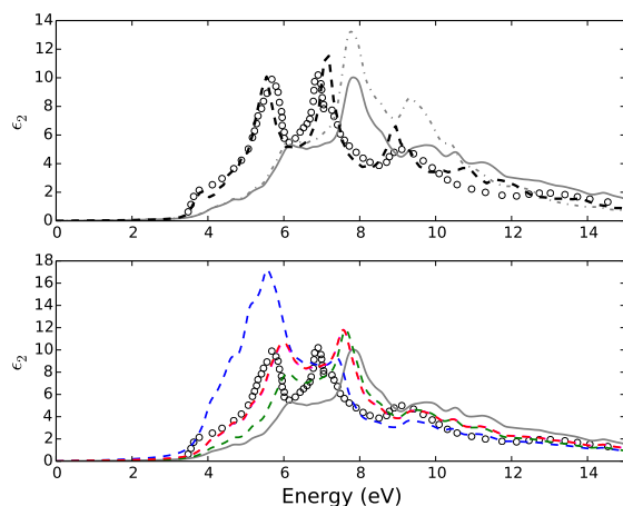
Figure 1 Optical absorption (imaginary part of the macroscopic dielectric function \varepsilon_2 ) in bulk ZnS. Top panel: experimental spectrum 19 (circles) compared with the independent particle (grey dashed-dotted line) and random phase approximation (grey continuous line) and Bethe-Salpeter equation (black dashed line). Bottom panel: experimental spectrum (circles) compared with the approximations for the polarisation functional described in Sec. 2, \alpha^{\text{EMP}}\mathbf{P} (red dashed line), \alpha^{\text{BER}}\mathbf{P} (magenta dashed line), \alpha^{\text{ED}}\mathbf{P} (green dashed line) and \alpha^{\text{IGM}}\mathbf{P} (blue dashed line). For reference the random phase approximation is also shown (grey continuous line).
