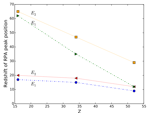
Figure 9 Redshift with respect the RPA results of the E_1 and E_2 peaks position in \epsilon_2 as a function of the chalcogen anion atomic number Z (and of the static macroscopic dielectric constant \epsilon_M(0) within the Bethe-Salpeter equation framework) for the Bethe-Salpeter equation (orange squares, E_2 , and green right triangles, E_1 ) and the polarisation functional with \alpha^{\text{EMP}} (red left triangles, E_2 , and blue circles, E_1 ). Lines between points are a guide for the eye.
