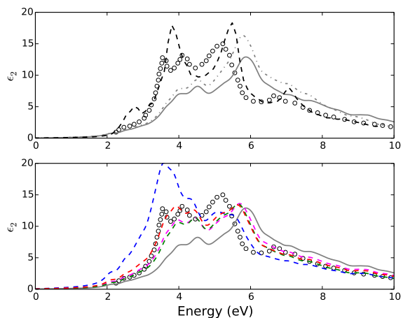
Figure 4 Optical absorption (imaginary part of the macroscopic dielectric function \epsilon_2 ) in bulk ZnTe. Top panel: experimental spectrum 22 (circles) compared with the independent particle (grey dashed-dotted line), random phase approximation (grey continuous line) and Bethe-Salpeter equation (black dashed line). Bottom panel: experimental spectrum (circles) compared with the approximations for the polarisation functional described in Sec. 2, \epsilon^{\text{xc}} \approx \alpha^{\text{EMP}}\mathbf{P} (red dashed line), \epsilon^{\text{xc}} \approx \alpha^{\text{BER}}\mathbf{P} (magenta dashed line), \epsilon^{\text{xc}} \approx \alpha^{\text{ED}}\mathbf{P} (green dashed line) and \epsilon^{\text{xc}} \approx \alpha^{\text{JGM}}\mathbf{P} (blue dashed line). For reference the random phase approximation is also shown (grey continuous line).
