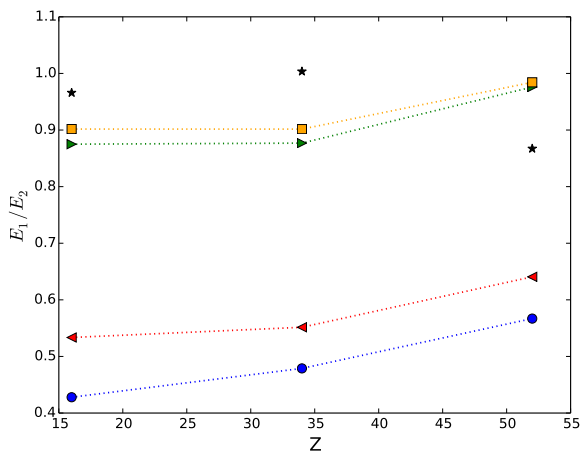
Figure 7 E_1/E_2 ratio of peak intensities in \epsilon_2 as a function of the chalcogen anion atomic number Z in calculations at Bethe-Salpeter (yellow squares), TD-DPFT with the \alpha^{\text{EMP}} \mathbf{P} functional (green right triangles), RPA (red left triangles) and independent particle (blue circles) level. Experimental ratios are reported for comparison (black stars). Lines between points are a guide for the eye.
