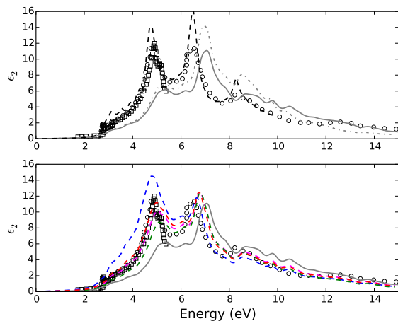
Figure 3 Optical absorption (imaginary part of the macroscopic dielectric function \epsilon_2 ) in bulk ZnSe. Top panel: experimental spectrum at room temperature 21 (circles) and at 20K 21 (squares) are compared with the independent particle (grey dashed-dotted line), random phase approximation (grey continuous line) and Bethe-Salpeter equation (black dashed line). Bottom panel: experimental spectra (circles and squares) are compared with the approximations for the polarisation functional described in Sec. 2, \epsilon^{\text{xc}} \approx \alpha^{\text{EMP}}\mathbf{P} (red dashed line), \epsilon^{\text{xc}} \approx \alpha^{\text{BER}}\mathbf{P} (magenta dashed line), \epsilon^{\text{xc}} \approx \alpha^{\text{ED}}\mathbf{P} (green dashed line) and \epsilon^{\text{xc}} \approx \alpha^{\text{JGM}}\mathbf{P} (blue dashed line). For reference the random phase approximation is also shown (grey continuous line).
