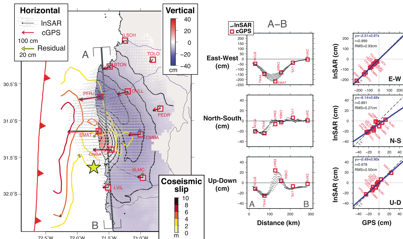
Figure 4. (left) Three-dimensional surface displacement reconstructed from Sentinel-1 InSAR. Red arrows show displacement at continuous GPS sites (cGPS), while color fill in red squares interior represents the vertical component of displacement from GPS (S. Ruiz et al., under review, 2016). Black arrows show displacement deduced from Sentinel-1 InSAR at locations of GPS benchmarks. Residuals are shown in yellow, with enhanced scaling. Grey arrows show horizontal displacement sampled on a regular grid. The colored grid in the background shows the vertical component of displacement on the same regular grid, with contours at 5 cm interval overlaid. Coseismic slip contours from the U.S. Geological Survey are shown for comparison ( http://earthquake.usgs.gov/earthquakes/eventpage/us20003k7a#scientific_findefault ). (middle) Transect showing comparison between Sentinel-1 InSAR and GPS. Location of the profile is shown in Figure 4 (left). East-west component (top), north-south component (middle), and vertical component (bottom). Sign convention is right-handed ENU. Note the different scaling for the east-west component. (right) Linear regression between Sentinel-1 InSAR and GPS displacements at GPS sites.
