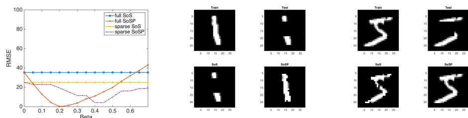
(a) Mean over all the test, l = 10 (b) Reconstruction with a full network, l = 20 , \beta = 0.05 (c) Reconstruction with a sparse network, l = 20 , \beta = 0.15
