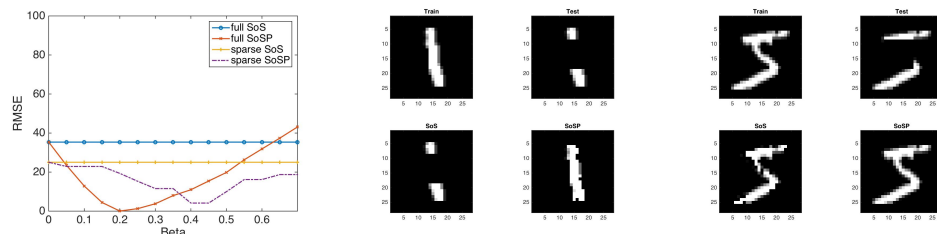
(a) Mean over all the test, l = 10 with 30 images learned (b) Reconstruction with a full network, l = 20 , \beta = 0.05 (c) Reconstruction with a sparse network, l = 20 , \beta = 0.15
