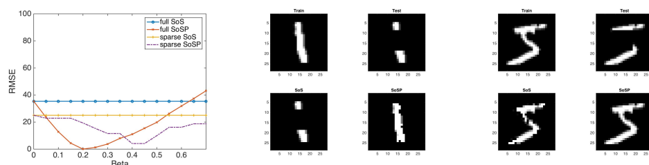
(a) Mean over all the test, l = 10 with 30 images learned (b) Reconstruction with a full network, l = 20 , \beta = 0.05 (c) Reconstruction with a sparse network, l = 20 , \beta = 0.15
