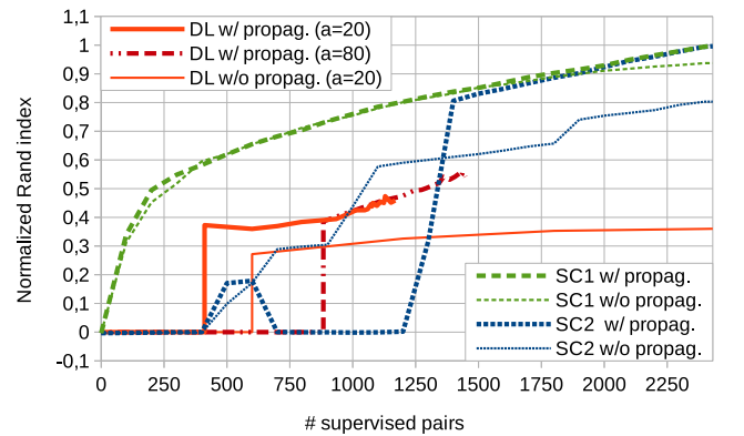
Fig. 11. Active semi-supervised clustering with (and without) propagation on Technology and Music genres of the MediaEval dataset (2431 videos - 2 classes).
