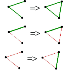
Fig. 4. Pairwise constraints propagation in a 2-classes problem.
