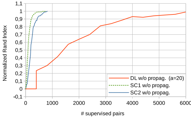
Fig. 8. Active semi-supervised clustering without propagation on Sonar dataset (208 objects - 2 classes).
