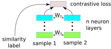
Fig. 5. Typical siamese architecture [8]
