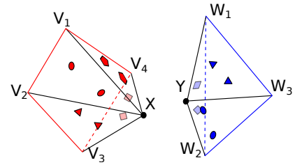
(a) The original neighborhoods of two vertices before ring join.
