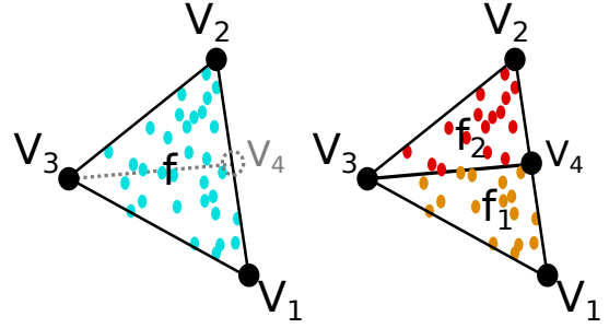
Figure 3: Splitting an edge at its center. Left: CompEls in f before split. Right: Distribution of CompEls between f_1 and f_2 after V_4 splits the edge V_1V_2 at its center.
