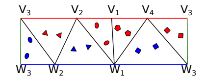
(c) Resulting connectivity unwind at the edge V_3W_3 (shown in green, duplicated)
