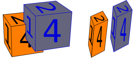
(b) A hypothetical side view before (left) and after (right) squish reveals that the two intersecting CompEls had their vertices moved towards the depth of their respective centers of mass in the NDC.
