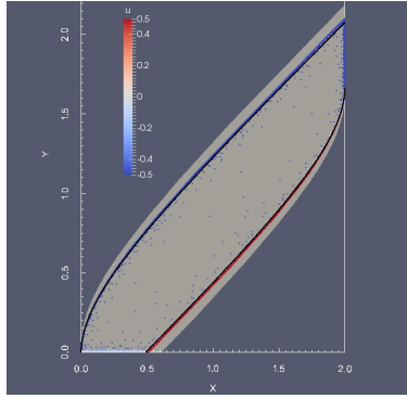
Figure 2: Approximation of the viability kernel for the consumption problem with parameters b = 2 , d = 3 , c = 0.5 , depth=20 (1024 points per axis), dt = 0.05 (integration step 0.001), 0.1. for the control discretization step. In gray the viability kernel with basic dilation parameter \nu = 2 . Colored points are the testing points of the leaves of the approximation with \nu = 0 . The color stands for the value of the control u . In black color points of the boundary of the true kernel
