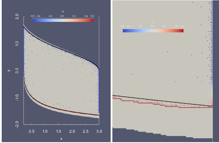
Figure 1: Approximation of the viability kernel with 1024 points / axis for the population problem with constraint set K = [a = 0.2, b = 3] \times [d = -2, e = 2] , parameters dt = 0.1 (integration step 0.01), control set U = [-0.5; 0.5] with discretization step 0.02. In gray the approximated viability kernel with dilation parameter \nu = 1 . Colored points are testing points of the leaves of the approximation with \nu = 0 . The color stands for the value of the control u . In black the boundary of the true kernel. Detailed view on the right.
